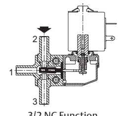
3/2 NC Function
