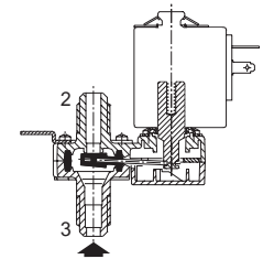
2/2 NC Function
