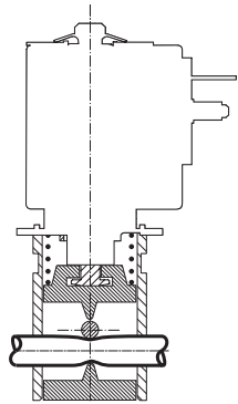
2/2 Normally Open
