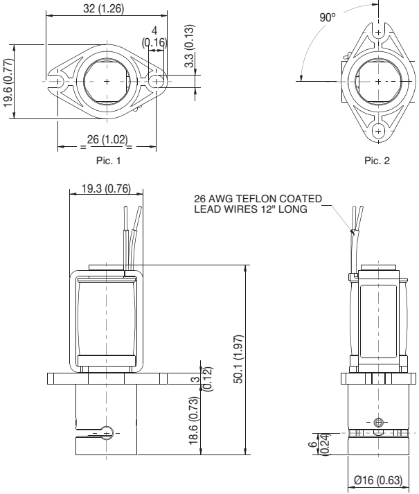
2/2 Normally Open
