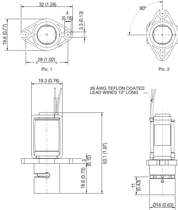
2/2 Normally Closed
