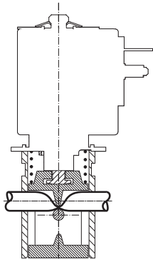
2/2 Normally Closed
