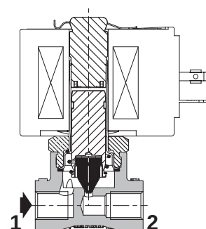
NC function (263 - 1/8)
