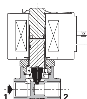
NC function (262 - 1/4)
