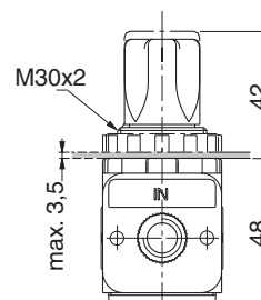
Panel mounting hole dia. 30,5
