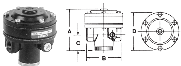
50 Series Pilot Operated Regulator (02,03,04)
