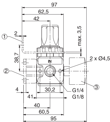
Mounting with bracket(s)
