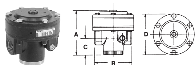
50 Series Pilot Operated Regulator (06,08)
