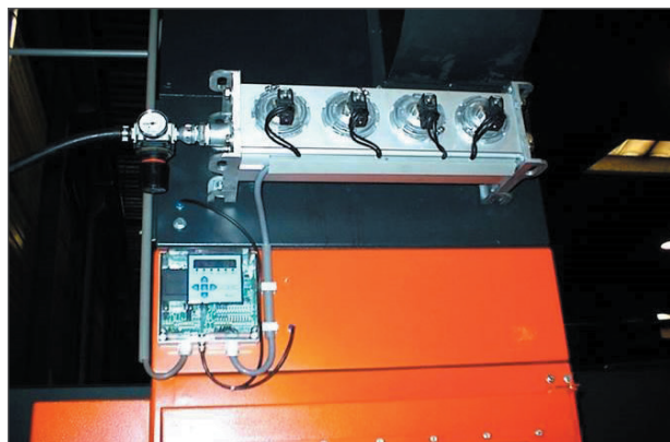
Aluminium tank system with integrated power pulse valves 1" and sequencer of ASCO (Series E909).
