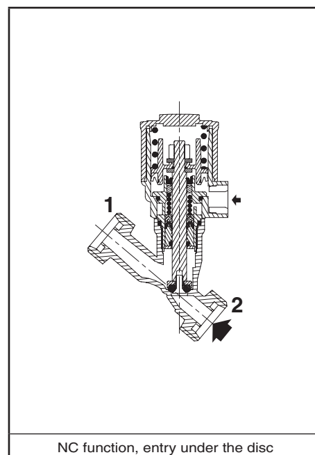
NC function, entry under the disc
