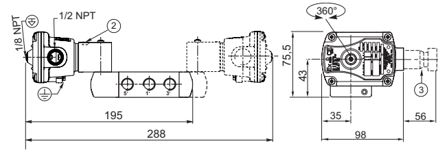
TYPE 03: No prefix, IP65 [551 suffixes: GD (II 1 GD c) ; SL (SIL) ; GDSL (SIL, II 1 GD c) 553 suffixes: GD (II 2 GD c) ; SL (SIL) ; GDSL (SIL, II 2 GD c)] Air operated version
