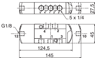
TYPE 03: No prefix, IP65 [551 suffixes: GD (II 1 GD c) ; SL (SIL) ; GDSL (SIL, II 1 GD c) 553 suffixes: GD (II 2 GD c) ; SL (SIL) ; GDSL (SIL, II 2 GD c)] Air operated version
