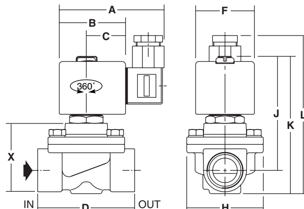
TYPE 02 Prefix "SC" Solenoid Epoxy moulded IEC 335 / ISO 4400 IP65 SCE030B003/B043
