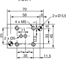
View F
