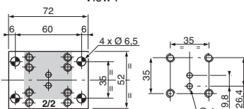
View F
